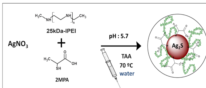
Figure 1. Schematic representation of the Ag 2 S@2MPA/LPEI synthesis.
